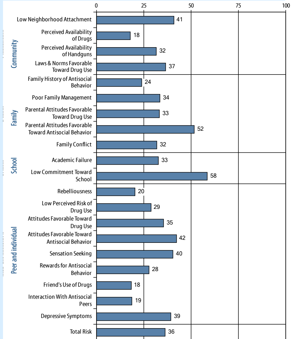
Butler County Risk Factors, 2023 Pennsylvania Youth Survey
